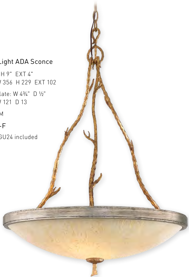
66-43 Four-Light Pendant W 24 1 / 2 " H 33 1 / 2 " mm: W 622 H 851 Canopy: W 5 1 / 2 " H 3/4" mm: W 140 H 19 4 / 100 M 66-43-F 4 / 26 GU24 included
